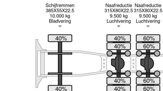
Scania S650 V8, EPSILON S290 Z 96. DOLL TRAILER... 6x4
