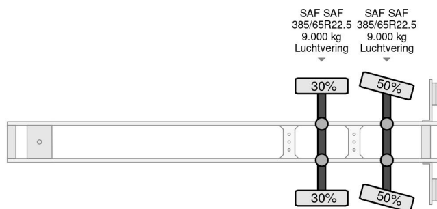
System Trailer TFSSH 18 TRPLY - 2 AXLE SAF + STEERING ...
