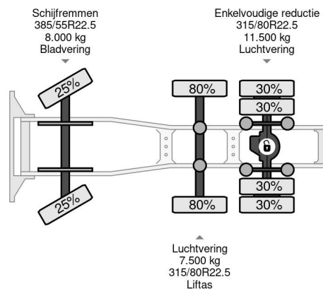
Volvo FH 460 6X2 - EURO 6 + LIFTING AXLE
