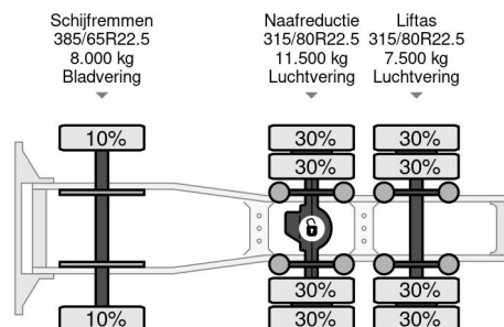
Volvo FH 540 6X2 - EURO 5 + BIG AXLE + LIFTING AXLE
