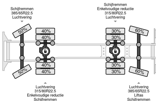
Volvo FH 460 8X4 - EURO 5 + CABLE LIFT
