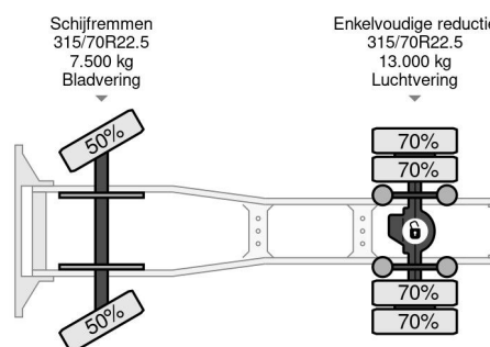
Volvo FM 330 4X2 - EURO 5 + CARRIER TRS - NL TRUCK
