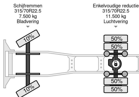
Scania R380 4X2 - SKIRTS + NL TRUCK - EURO 3 - 3 PEDALS
