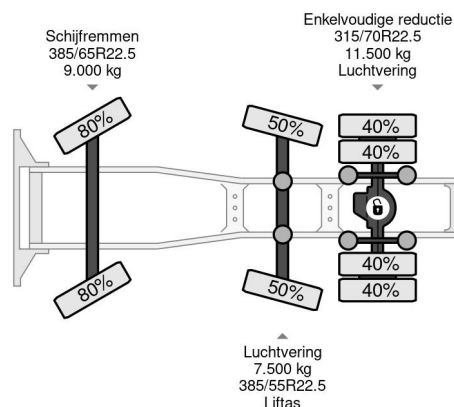
Scania R450 6X2 EURO 6 RETARDER LIFT + STEERING A...
