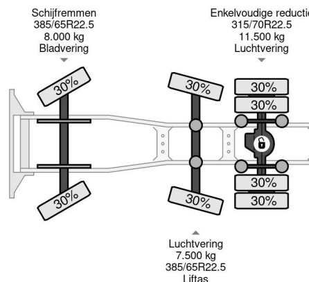
DAF XF 460 6X2 EURO 6 STEERING AXLE HYDRAULIC
