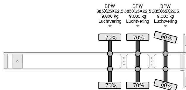
Sor 3 AXLE + CARRIER 1850 D/E
