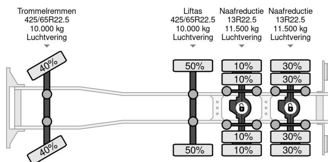
Terberg FM 1850 8X4 VDL HOOKLIFT EURO 5
