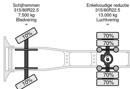
DAF CF 85.360 4X2 - EURO 5 - FULL SPOILER - NL TRUCK
