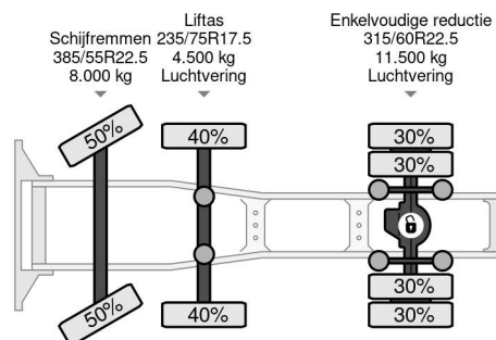
Scania R450 6X2 EURO 6 HYDRAULIC AUTOMATIC
