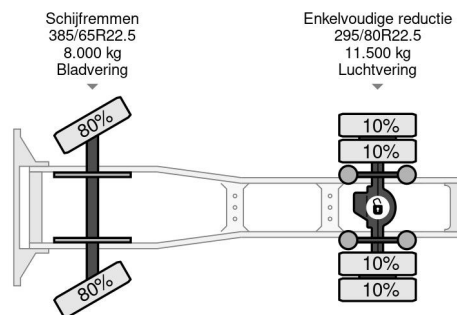
DAF XF 460 4X2 EURO 6 SKIRTS AUTOMATIC
