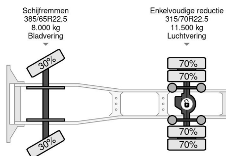
DAF XF 440 4X2 EURO 6 SKIRTS 2017
