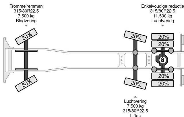
DAF 85.330 6X2 - VACUUM CLEANER + LIFT/STEERING A...
