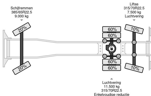
Scania P320 6X2 - EURO 6 + HIAB XS 144 HIPRO + REMO... Referentienummer: SC336154
