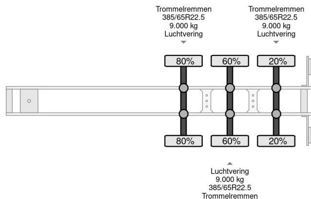
Pacton T3 004 - 3 AXLE
