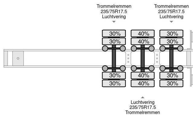
VS MONT VSAT 1103-3HM 3 TRUCKS + WINCH
