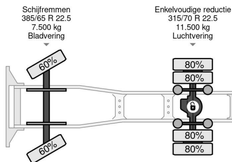
Volvo FH 460 4X2 EURO 6 i-Shift Low Roof APK
