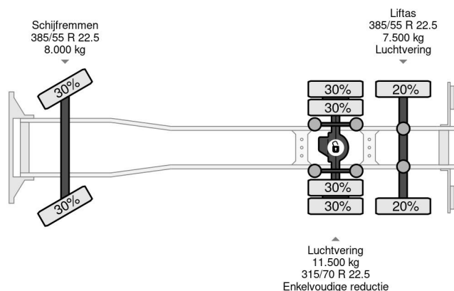
Volvo FH 460 6X2 EURO 5 CHASSIS
