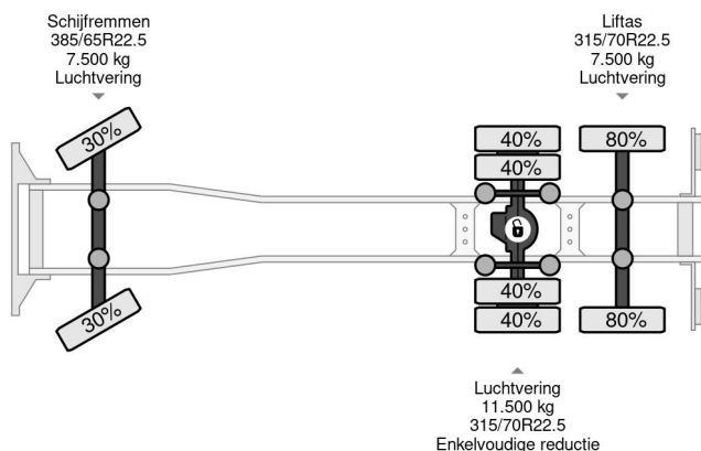
MAN TGS 26.440 6X2 - EURO 6 + THERMKING T-800R + D... Referentienummer: MA204489
