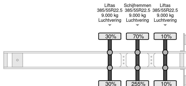
SCHMIDT HAGEN 3 AXLE + LIFTING AXLE
