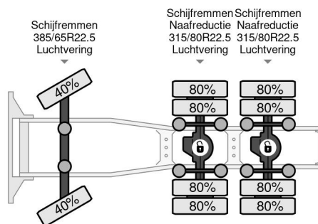
Volvo FH 540 6X4 - EURO 6 + PALFINGER EPSILON S260Z96
