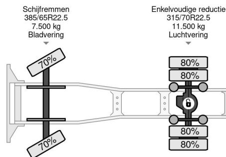
Renault T430 4X2 EURO 6 SKIRTS STANDKLIMA
