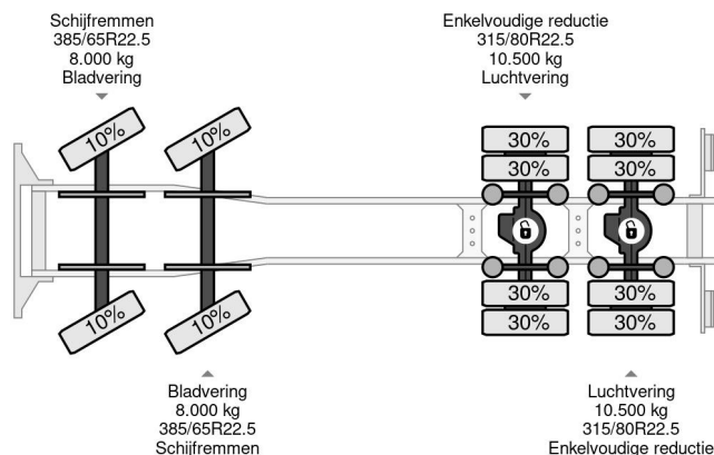
Volvo FH 500 8X4 - EURO 5 + CABLELIFT TIPPER
