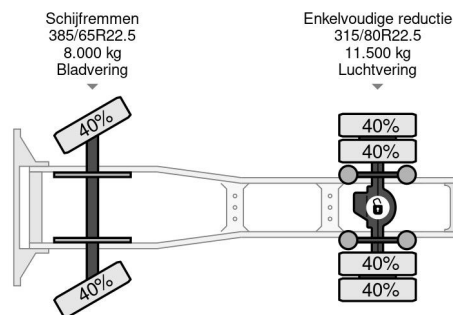
Volvo FH 16.600 4X2 ADR PARK COOL EURO 5 ALCOA
