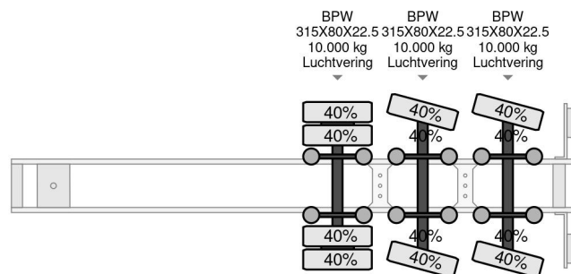
Floor LAST 2 AXLE STEERING, FIRST LIFT AXLE
