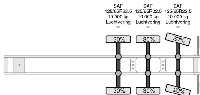
Pacton TBD 346 - 3X SAF AXLE + LIFTING + STEERING AX...
