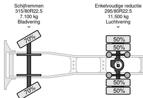
DAF CF 75.290 4X2 EURO 3 MANUAL GEAR
