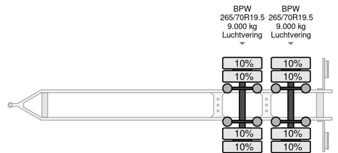
Burg M-2-18 - 2 AXLE BPW + CARRIER TRS + DHOLLANDIA...
