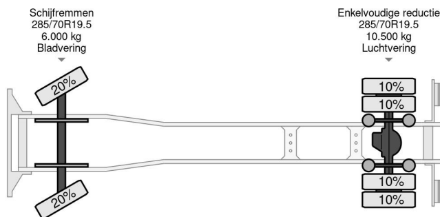
DAF LF 260 4X2 16T DHOLLANDIA LOAD LIFT
