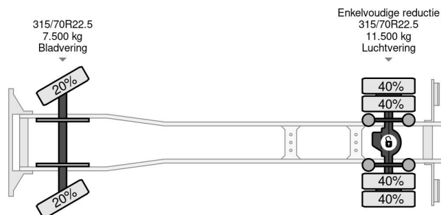
Volvo FL 619 4X2 + CARRIER SUPRA 550 + B.A.R CARGOLIFT
