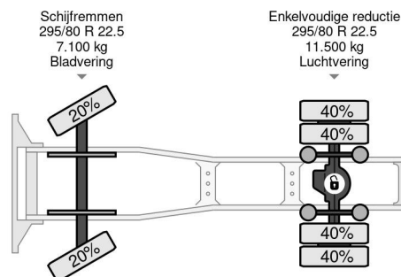
DAF XF 105.460 SC 4X2 EURO 5 MANUAL
