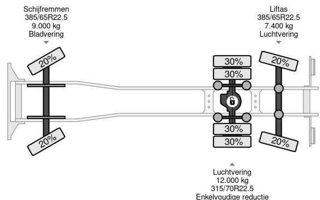
DAF XF 105.460 SSC 6X2 - EURO 5 - 793.995 KM - CHASSIS
