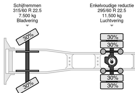
DAF XF 440 SC 4X2 EURO 6 MEGA
