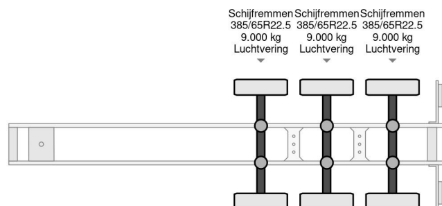
Atcomex 10 UNITS - 3 AXLE KIPPER BULK 1 COMP. 60.000... Referentienummer: AT121273-2
