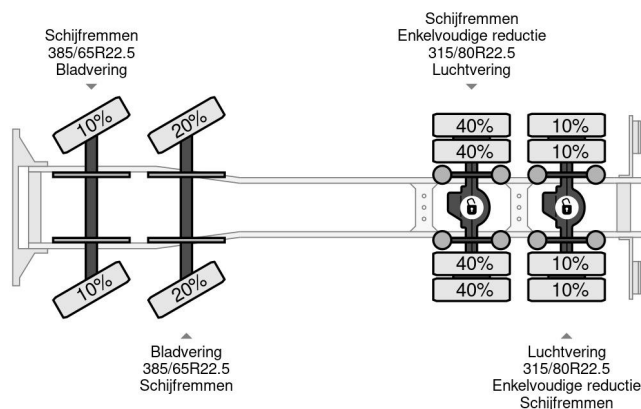
Volvo FM 440 8X4 EURO 5 + CABELLIFT TIPPER
