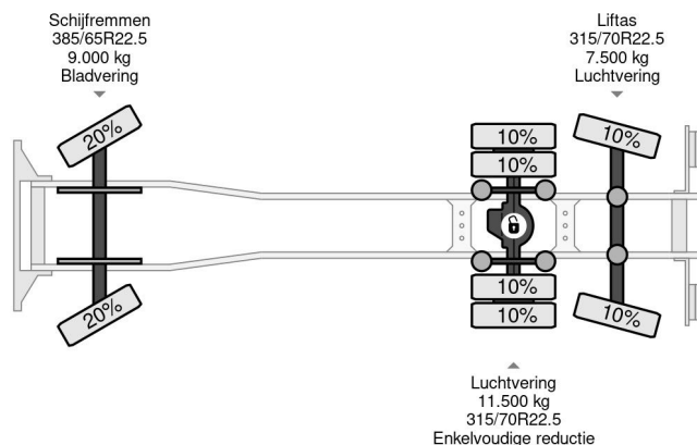
Volvo FM 370 6X2 VDL 21T + HIAB 211 + REMOTE CONTROL
