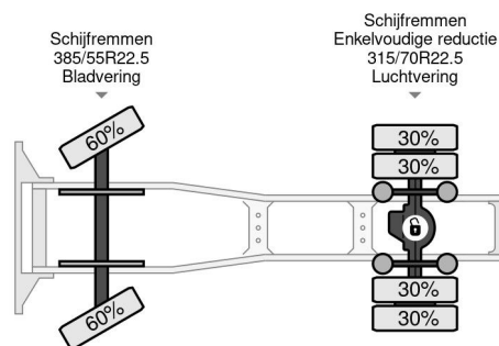
Scania R520 V8 4X2 NGS EURO 6 RETARDER SKIRTS
