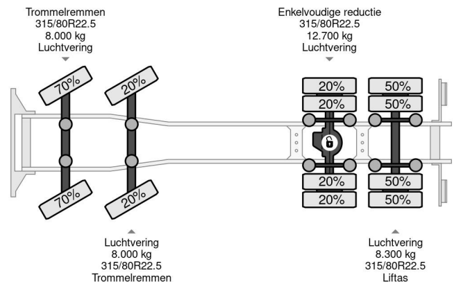
Scania R114-380 8X2 - EURO 3 + PM 23525SP LC 2013! + ...
