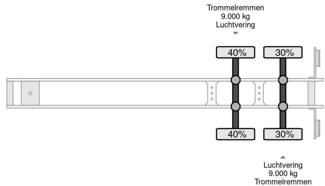
SYSTEM TRAILERS PRSH18 - 2 AXLE BPW
