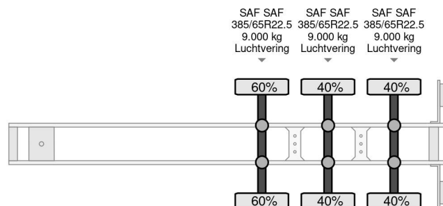
Burg BP0 12-27 - 3 AXLE SAF + LIFTING AXLE
