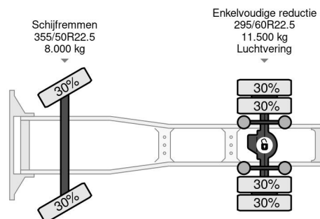
DAF XF 480 4X2 - EURO 6 + LOW DECK + FULL SPOILER
