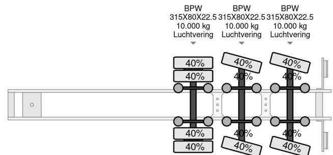
Floor LAST 2 AXLE STEERING, FIRST LIFT AXLE
