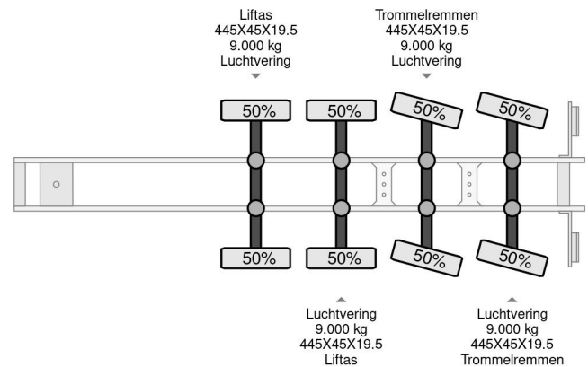
Floor 2 AXLE STEERING an 2 LIFT AXLE
