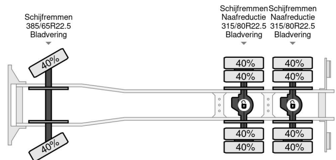
Volvo FM 420 6X4 EURO 5 FULL STEEL BIG AXLES AJK 20...
