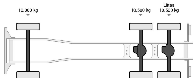
Volvo FH 540 6X4 - EURO 6 + HIAB XS 322 + REMOTE + LI...
