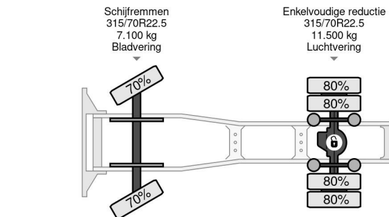
Scania P280 4X2 - EURO 6 + NL TRUCK
