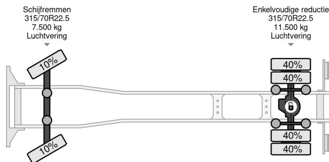
Volvo FH 460 4X2 TRS COOLING + BURG 2 AXLE HANGER
